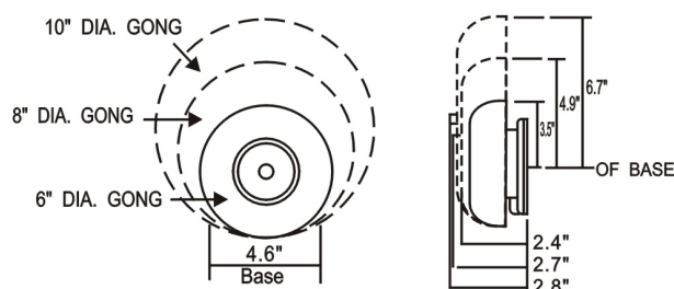
HC-1220 220 VAC
